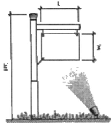
Freestanding Sign
